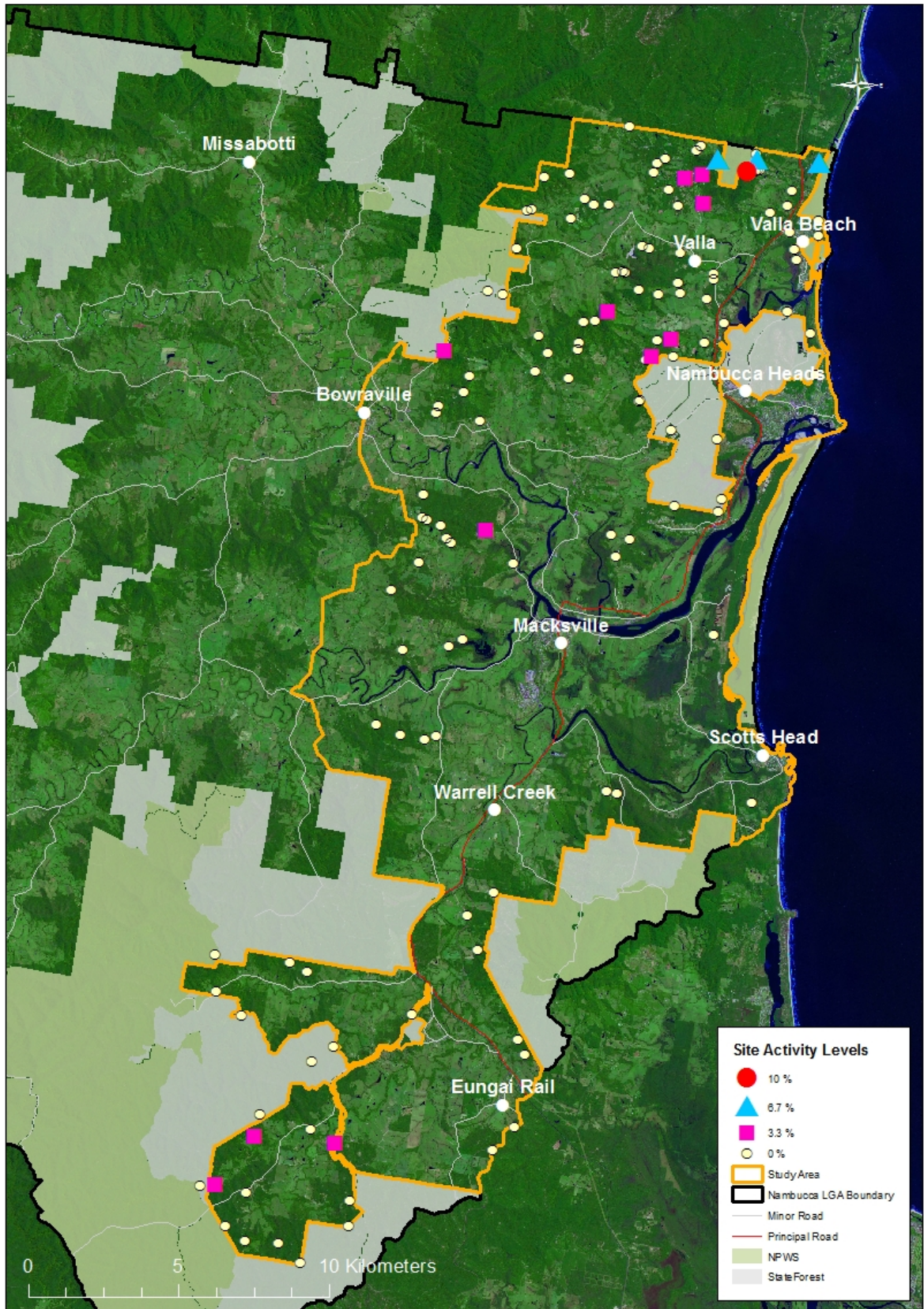
Map 7 Activity levels at sites where koala activity was recorded within the koala habitat study area.
